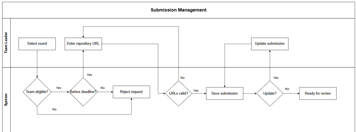
Figure 1.5 Submission Management Swimlane
