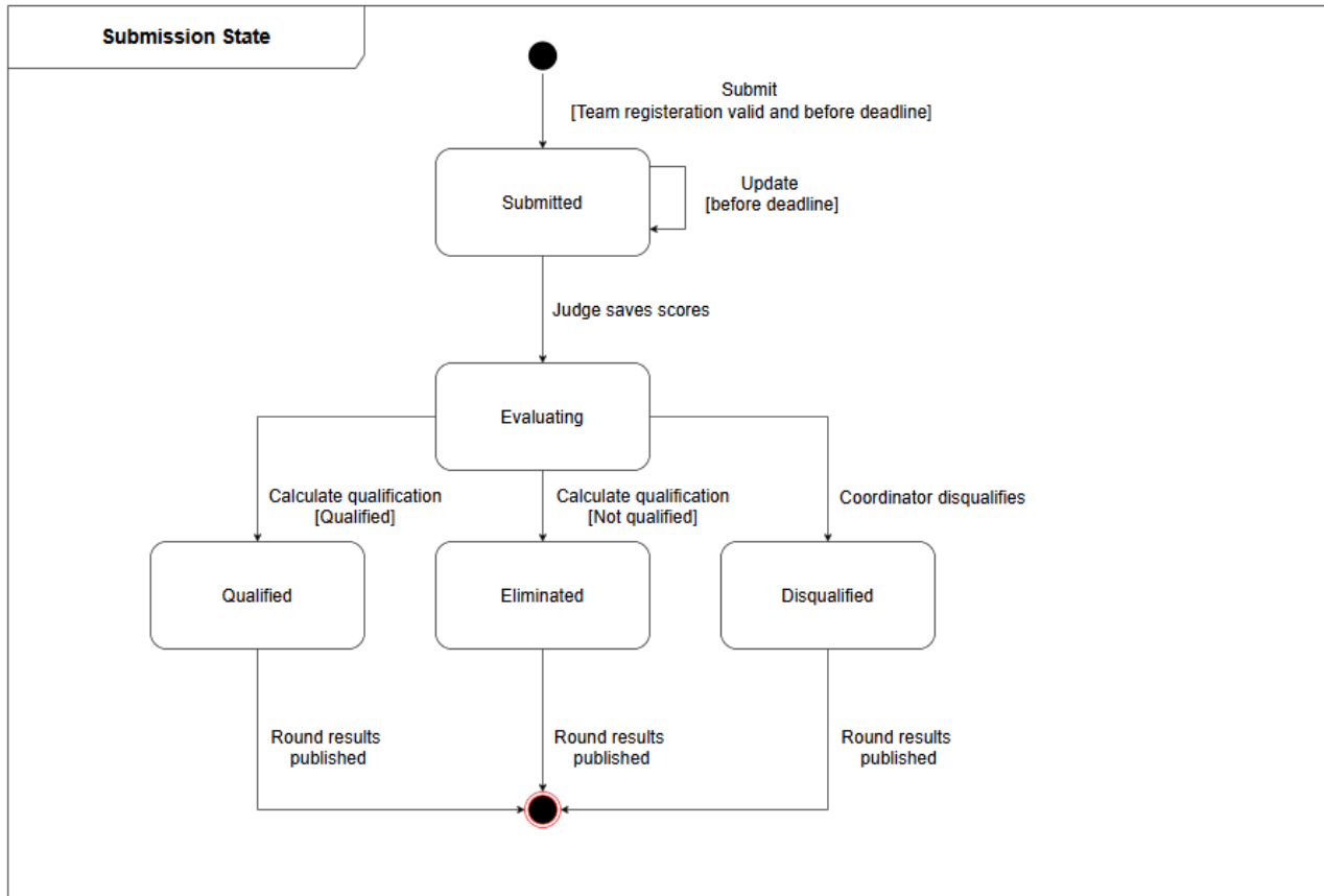
Figure 3.5 Submission State Chart
