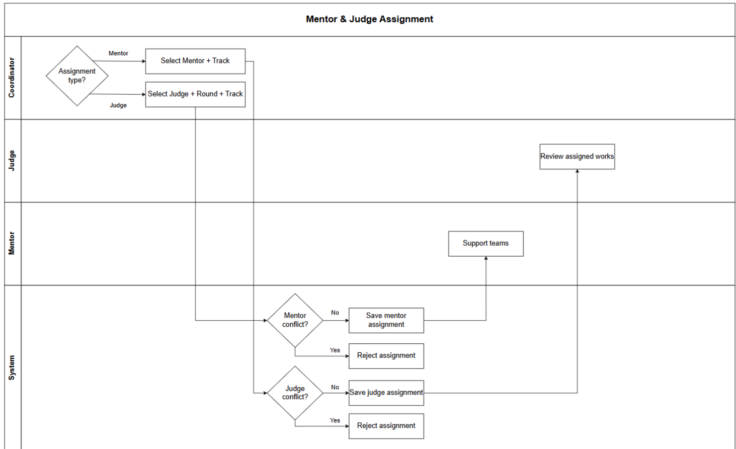
Figure 1.4 Mentor and Judge Assignment Swimlane
