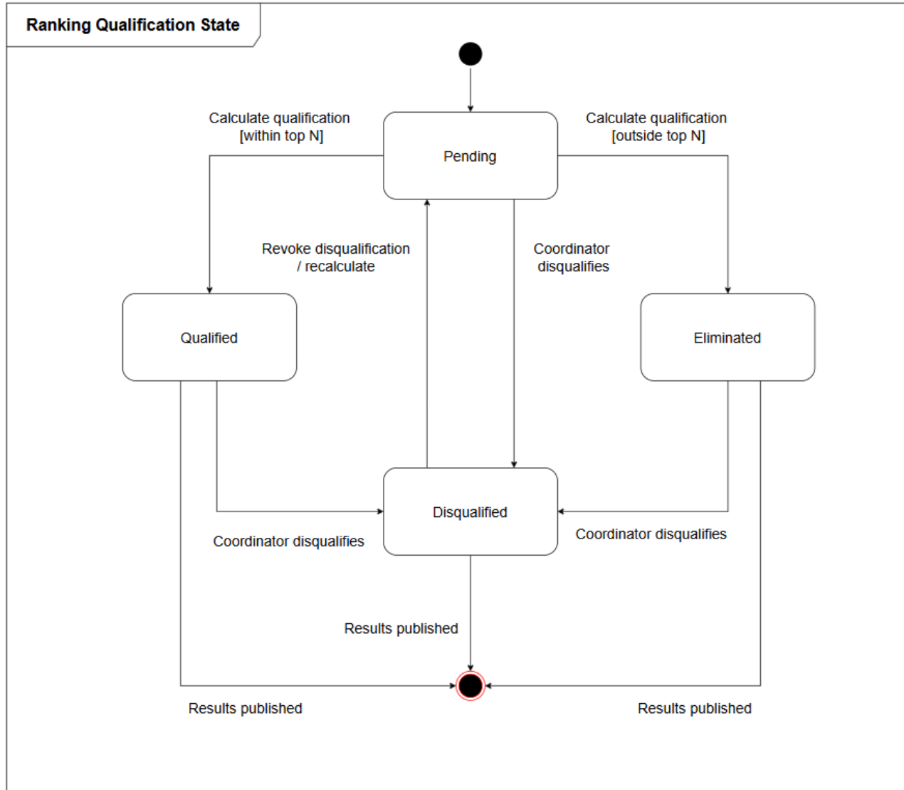
Figure 3.8 Ranking Qualification State Chart
